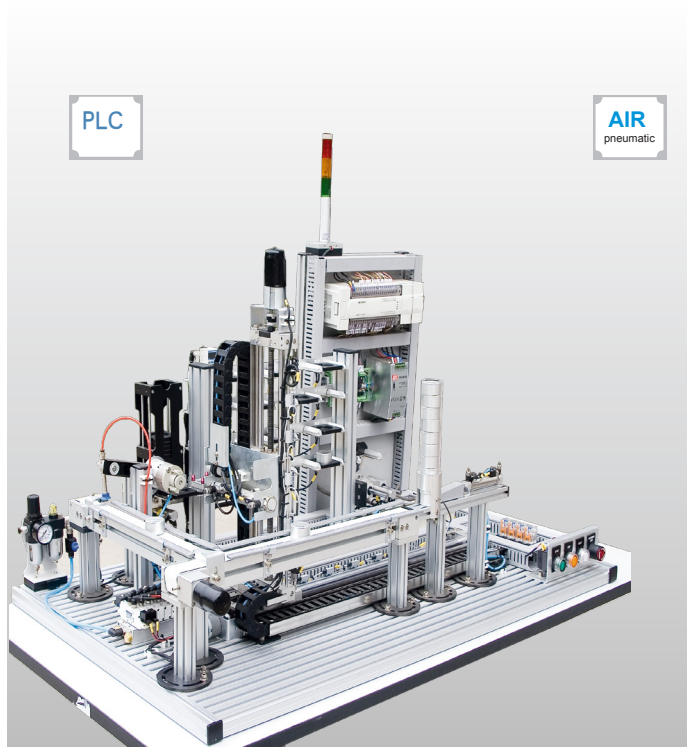
DLFA-ASRSA01 Automatic Storage and Retrieval System(Advanced)
