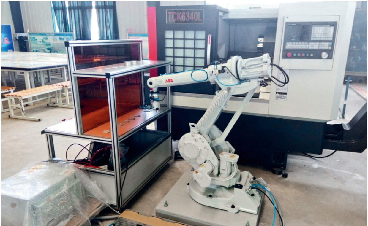
DLRB-1410A Industrial Robot CNC Machining Teaching Workstation
