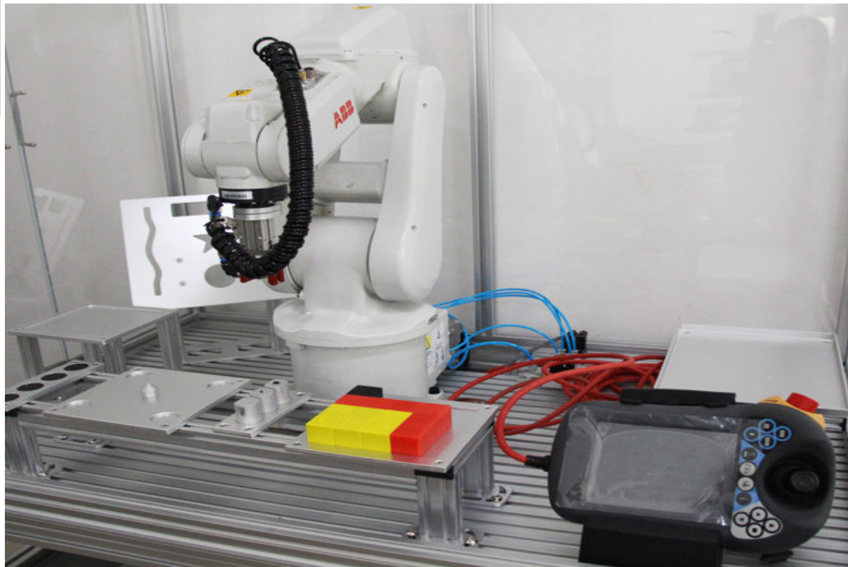
DLRB-120 Industrial Robot Basic Skills Training System
