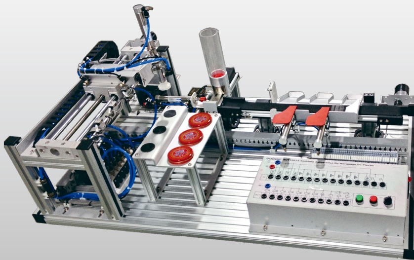
DLFA-BJJ03 Auto Marking Machine Training System
