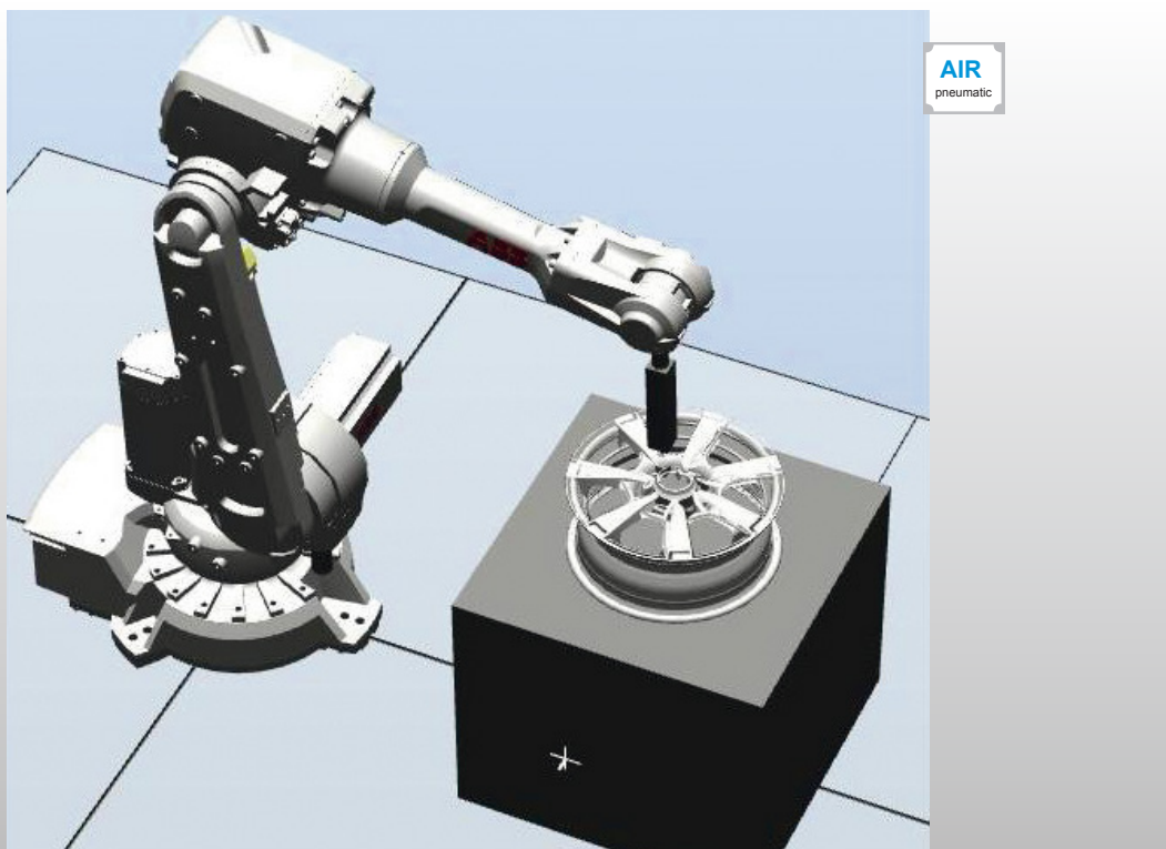
DLRB-2600 Robot Polishing Training System
