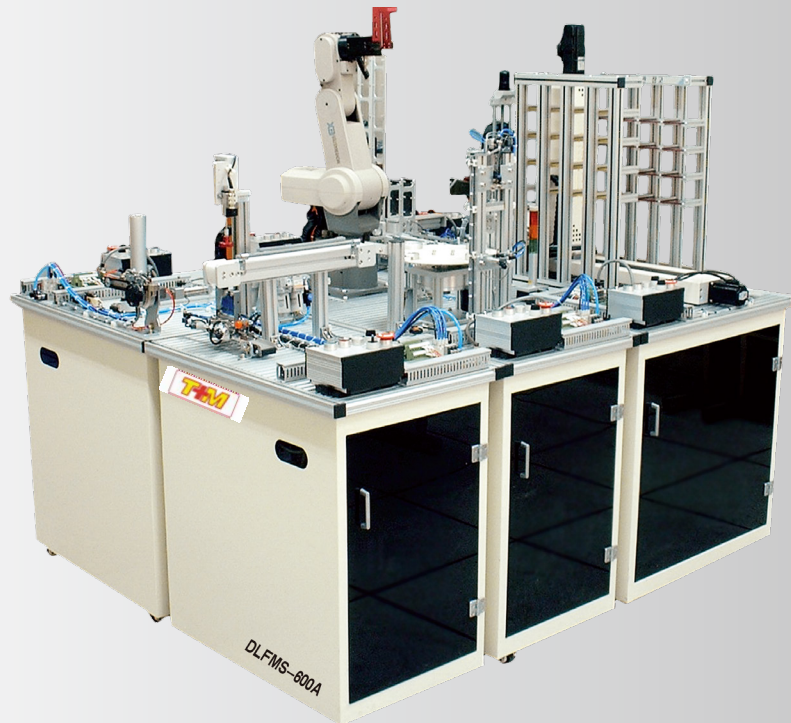
DLRB-600A Flexible Production Line Training System
