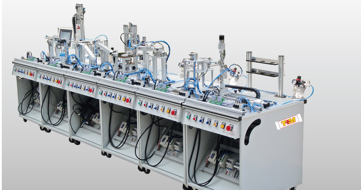
DLMPS-600A Modular Flexible Production Line Training System
