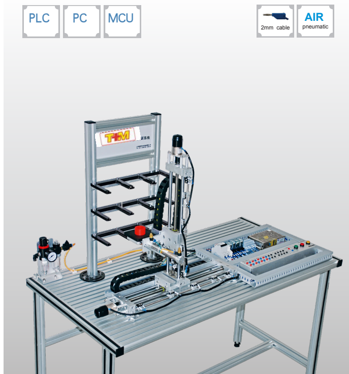
DLFA-ASRSB02 Automatic Storage and Retrieval System(Basic)
